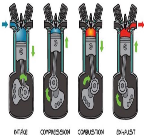
Four-stroke cycle (or Otto cycle)
